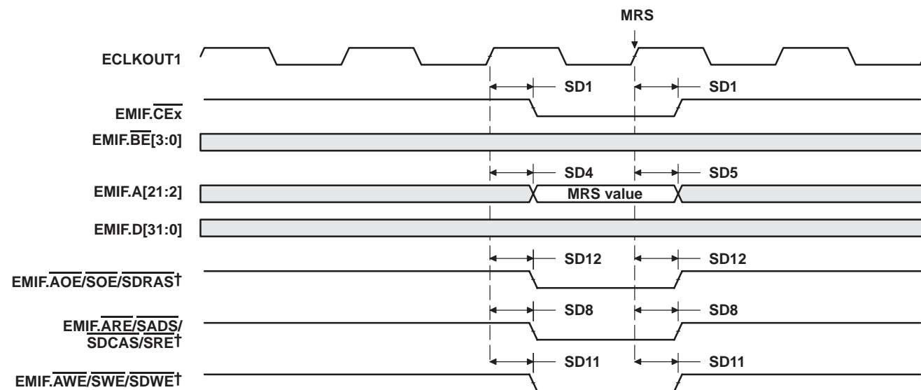
Figure 5–19. SDRAM MRS Command
